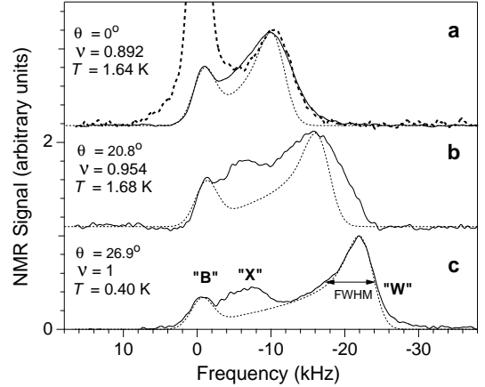
FIG. 1. Several ^{71}\text{Ga} OPNMR emission spectra (a-c, solid lines, offset for clarity), acquired at low T for different \nu , in B_{\text{tot}}=7.03 T ( f_o=91.36 MHz). The same “W” resonance is obtained using either conventional NMR absorption (a, dashed line) or OPNMR emission (a, solid line). The dotted lines (a-c) are fits to W and “B”, which assume identical quantum wells (see text).
